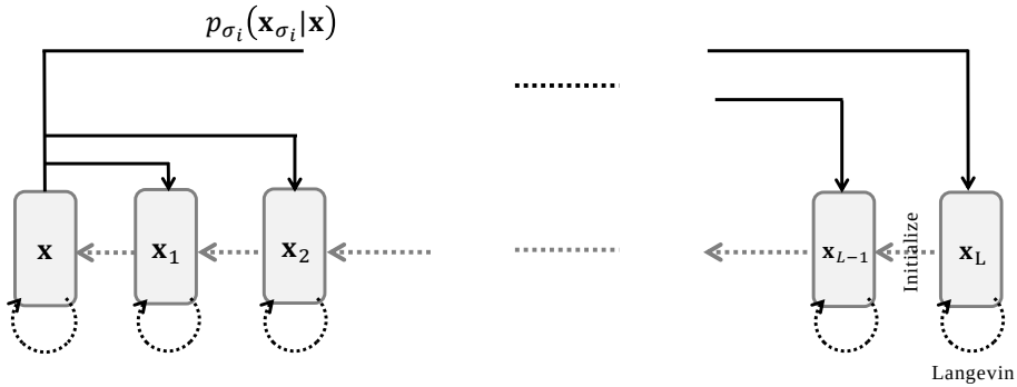
Figure 3.7: Illustration of NCSN. The forward process perturbs the data with multiple levels of additive Gaussian noise p_\sigma(\mathbf{x}_\sigma|\mathbf{x}) . Generation proceeds via Langevin sampling at each noise level, using the result from the current level to initialize sampling at the next lower variance.
