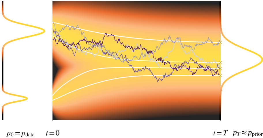
Figure 4.3: Visualization of the reverse-time stochastic process for data generation. It begins from samples drawn from a simple prior distribution ( p_{\text{prior}} ) at t = T (denoted as “ \times ”), which are evolved backward in time using a reverse-SDE. The resulting trajectories terminate at t = 0 and collectively form the target bimodal data distribution ( p_0 = p_{\text{data}} ). The background heatmap illustrates how the probability density is gradually transformed from a simple Gaussian into the complex target distribution.
