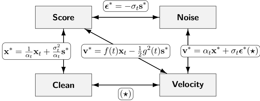
Figure 6.1: Equivalent relations among four parameterizations. \mathbf{v} -prediction is given by \mathbf{v}^* = \alpha_t \mathbf{x}^* + \sigma_t \epsilon^* , where clean and \epsilon -predictions are interchangeable via \mathbf{x}_t = \alpha_t \mathbf{x}^* + \sigma_t \epsilon^* .
